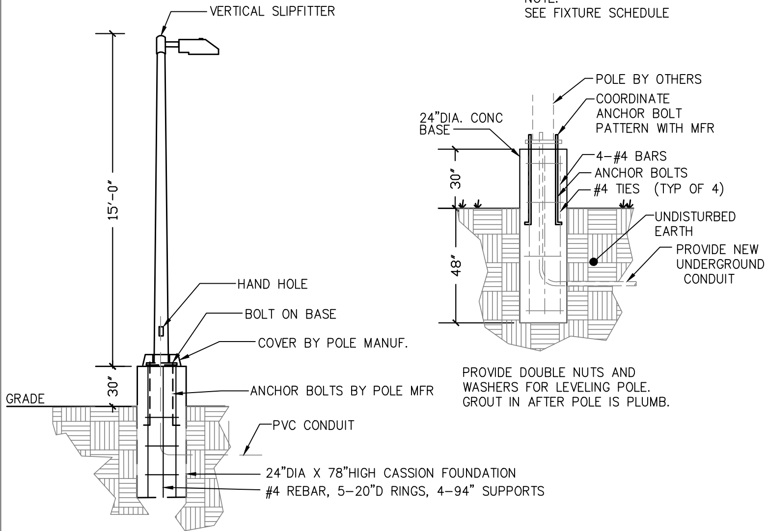
15FT BASE MOUNTED FIBERGLASS POLE WITH 30" AFG CAISSON
