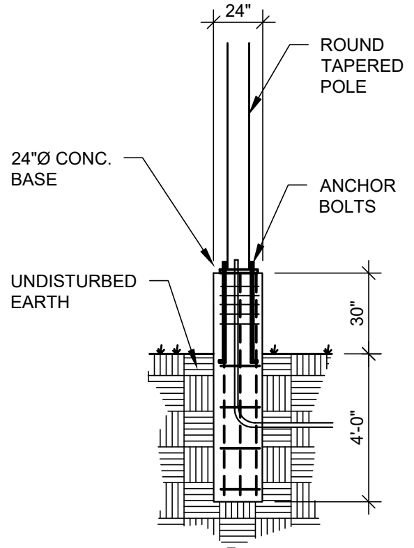
30' LIGHT POLE BASE
