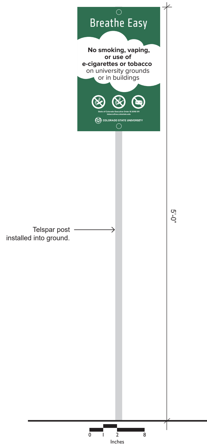
Signs mounted to posts (Light Posts and/or telespar posts) or buildings
